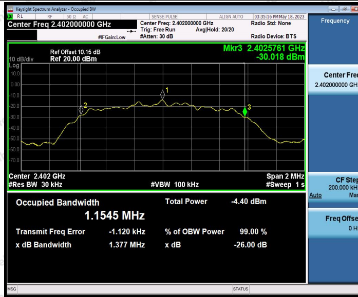
3DH1_Ant1_2441
